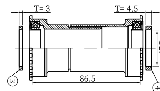
Road Wide _ 86.5L
