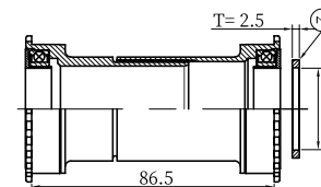
Road Wide _ 86.5L
